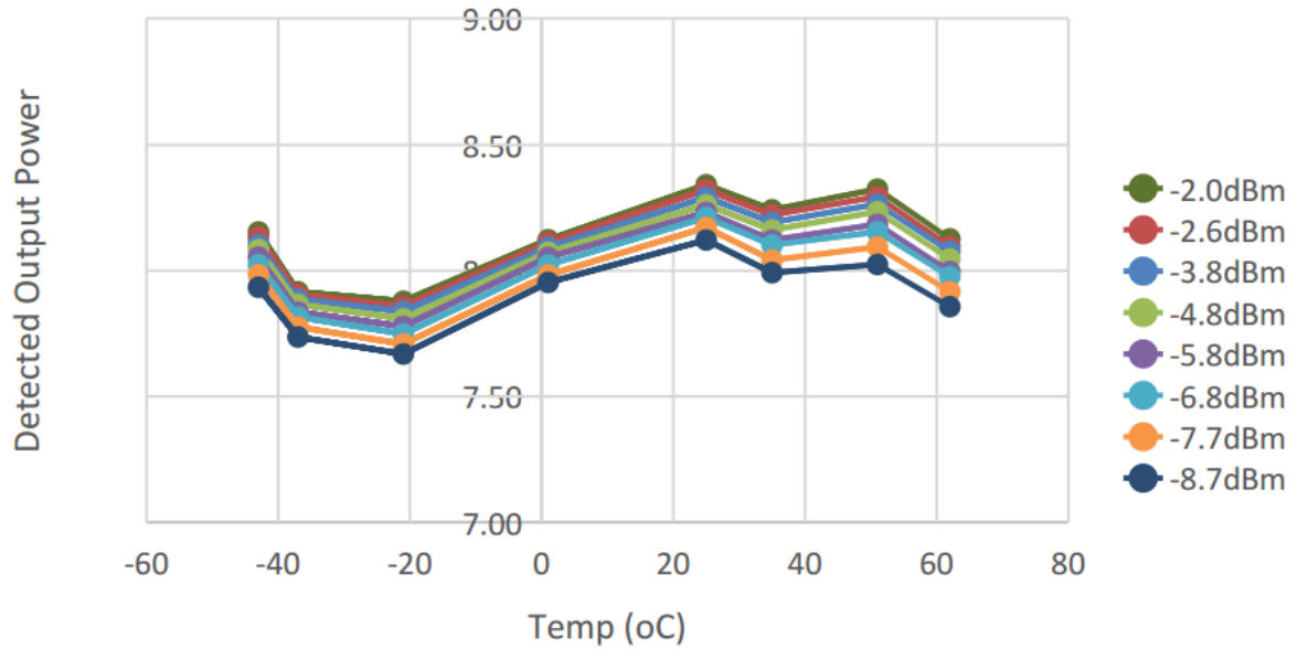
Output power for at least -2 dBm to -8 dBm input power
